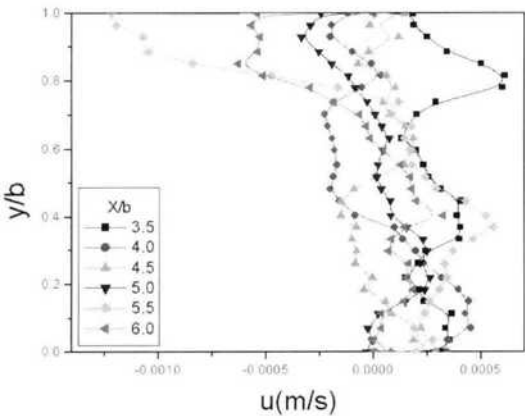
Fig. 18 Velocity distributions along the test tube for Re=0.62 with D.C 1.5kV/mm
