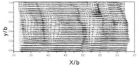
Fig. 14 Mean velocity vector distributions along the test tube for Re=1.29 with D.C 1.0kV/mm
