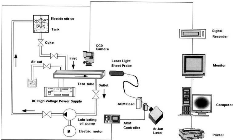
Fig. 2 Experimental apparatus and PIV system
