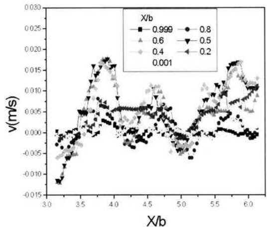
(b) Radial velocity distributions
