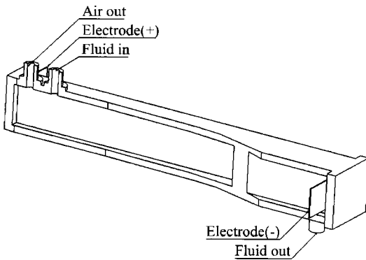
(a) Geometry of the test tube
