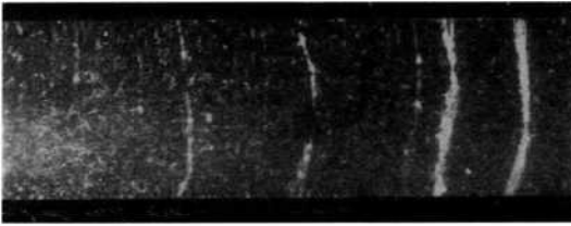
Fig. 16 Distributions of electro-rheological particles for Re=0.62 along the test tube with D.C 1.5kV/mm
