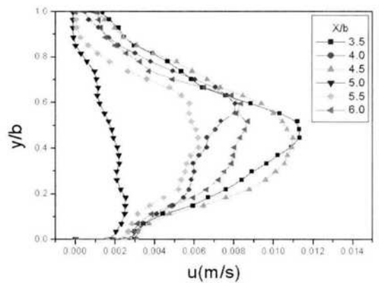
Fig. 15 Velocity distributions along the test tube for Re=1.29 with D.C 1.0kV/mm
