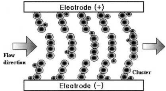
Fig. 19 Schematic clusters of ER fluid flow
